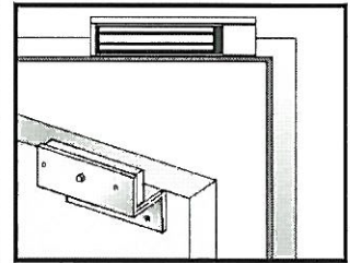
With LZ-bracket for in-swinging door frames
